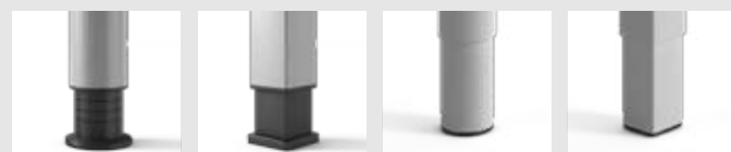
Round tube version (RR) plastic; Square tube version (RQ) plastic Round tube version (RR) tube in tube; Square tube version (RQ) tube in tube Height adjustment: Plastic: 680–820 mm; tube in tube: 620–850 mm
